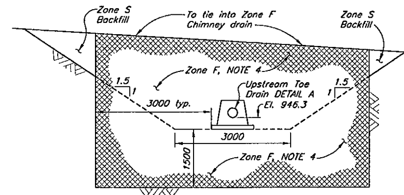
SECTION 1 - FILTER DIAPHRAGM Scale A
