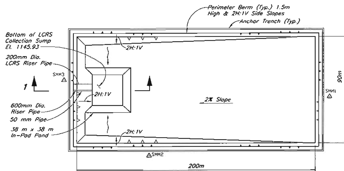
TEST HEAP LEACH PAD Scale A
