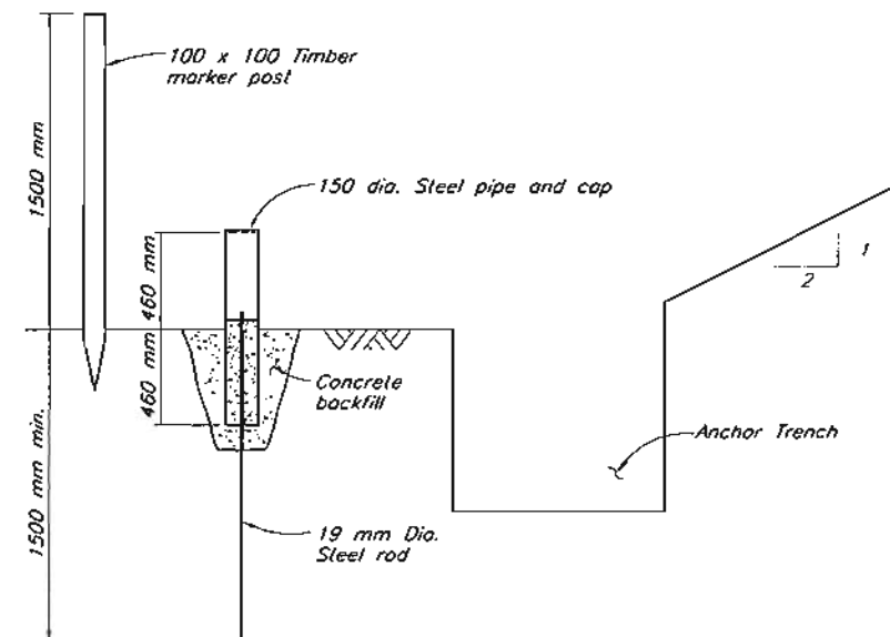
TYPICAL DETAIL OF SURFACE MOVEMENT MONUMENT Scale B
