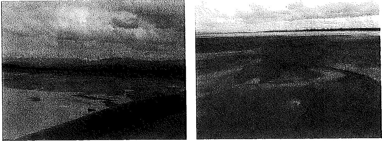
Photo 17 – Typical beach formed by single point discharge of tailings – overview and detail
