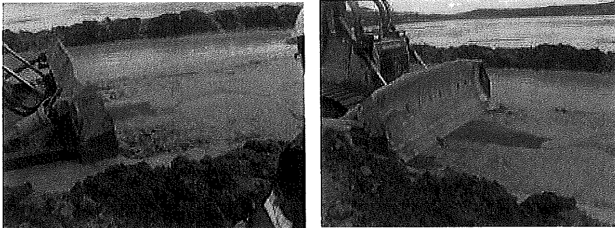
Photo 11 – Cell construction – pushing sand back
