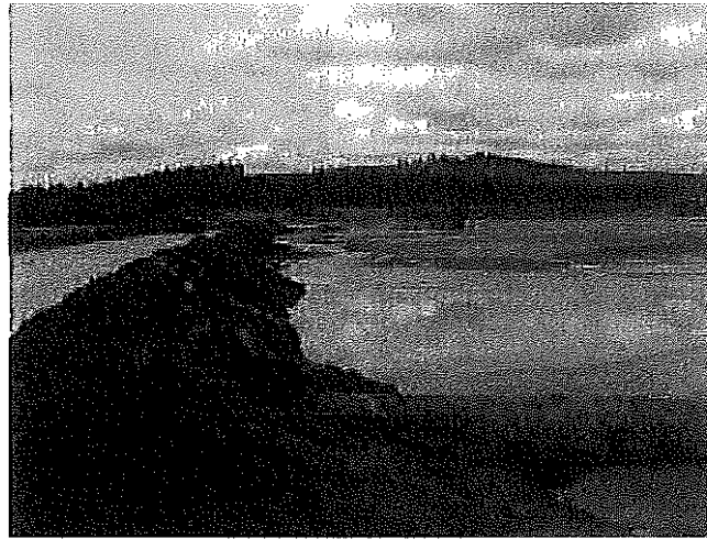
Photo 6 – Berm erosion by decant channel flow
