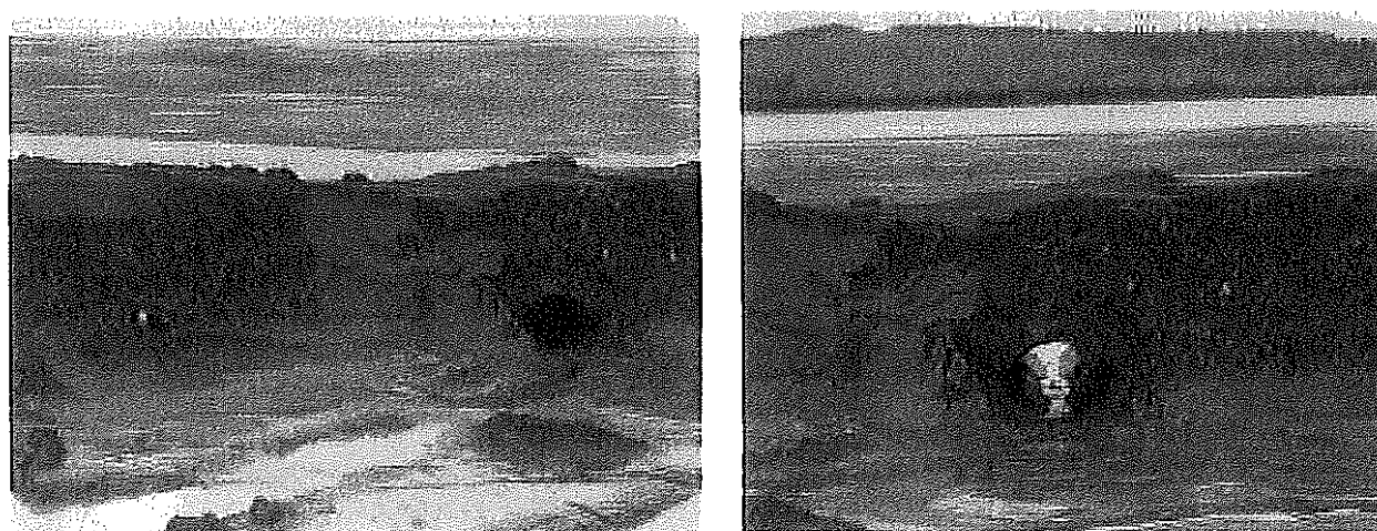
Photo 12 – Re-installed decant pipes
