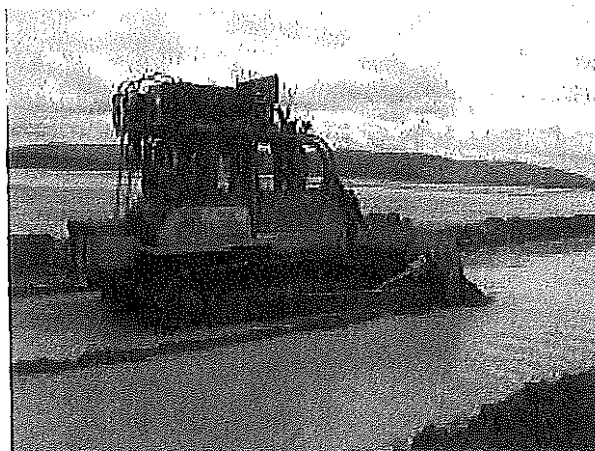
Photo 8 – Cell construction – pushing sand downstream
