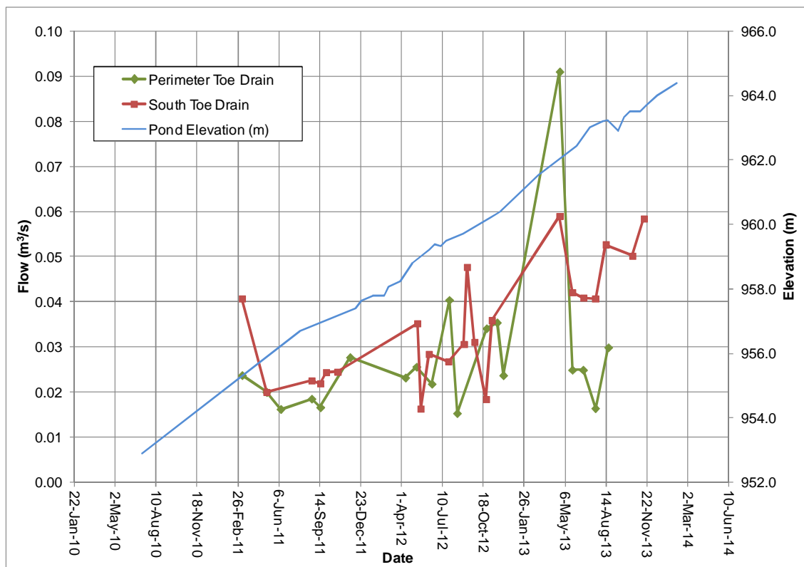
Figure 2.1: South and Perimeter Embankments Drain flow readings
