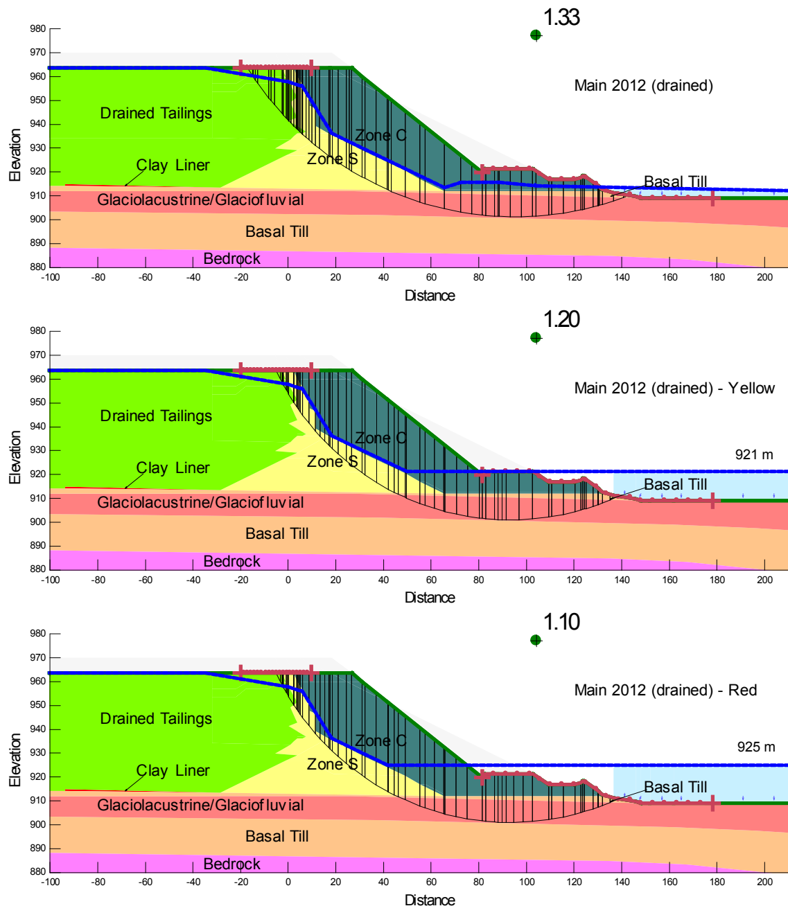
Figure 2.5: Pore Pressure Trigger Levels Stability Analysis
