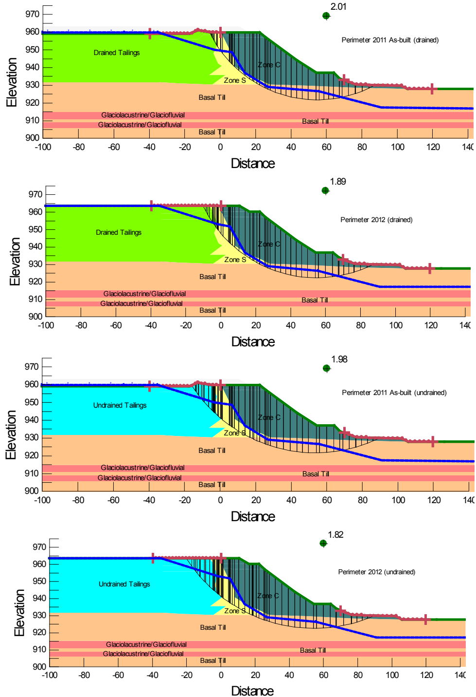
Figure 2.2: Perimeter Embankment Stability Analysis
